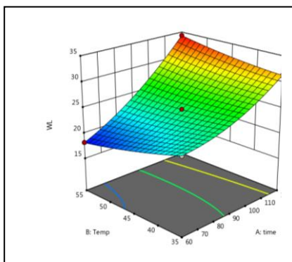
(a) immersion time and temperature
