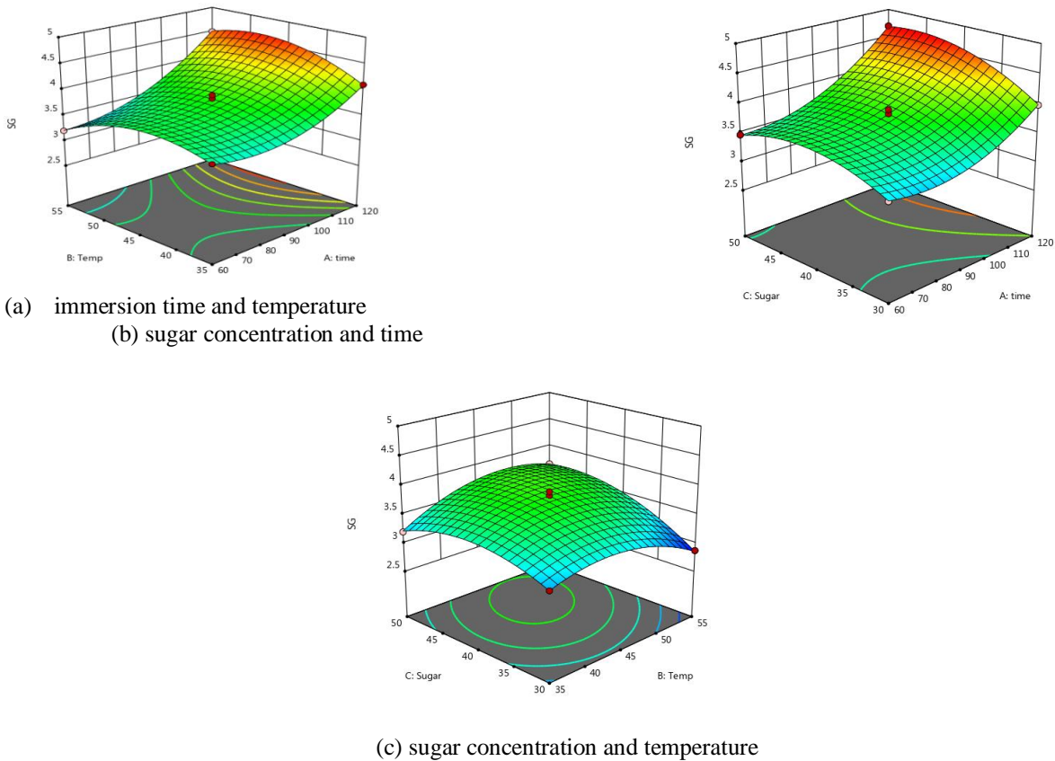
Fig 2. Solid gain during osmotic dehydration of toddy slices as a function of :
