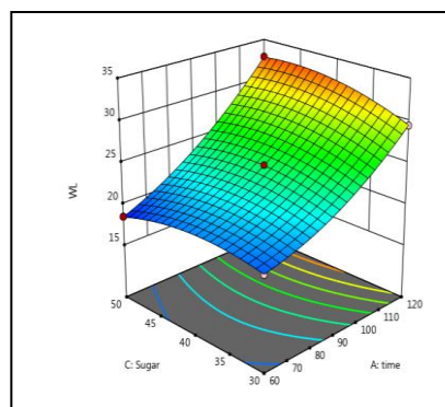
(b) sugar concentration and time
