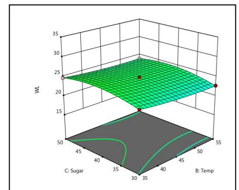
(c) sugar concentration and temperature
